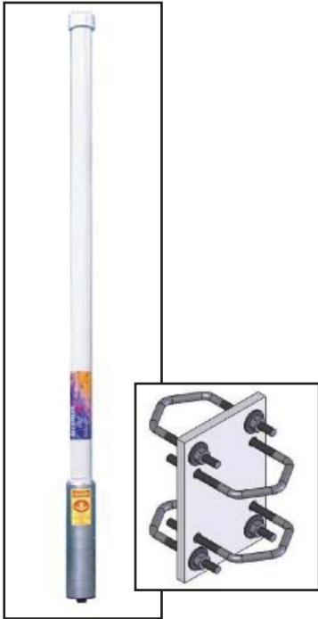
BGO902G (left) with BWC1005 clamp (right)
